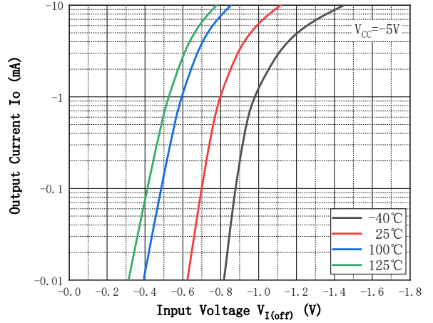
Fig.2 - OFF Characteristics
